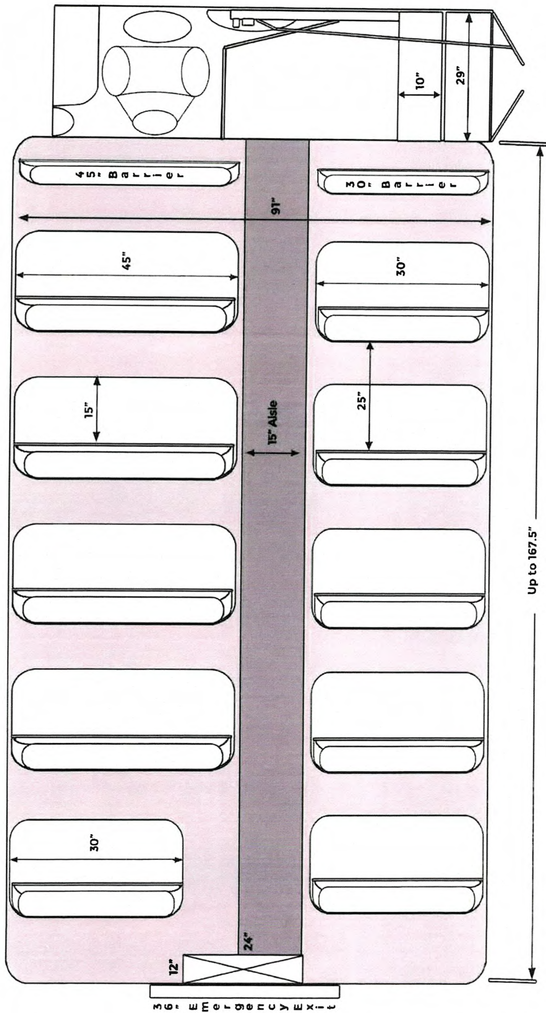
Floor Plan for 24 Passenger Seating Arrangement
